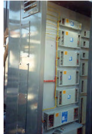
Stage 6 Installation of Tempest filters
