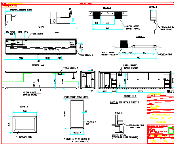
Stage 1 Full drawings for customer approval
